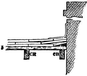
Section on E F, Fig. 260.
